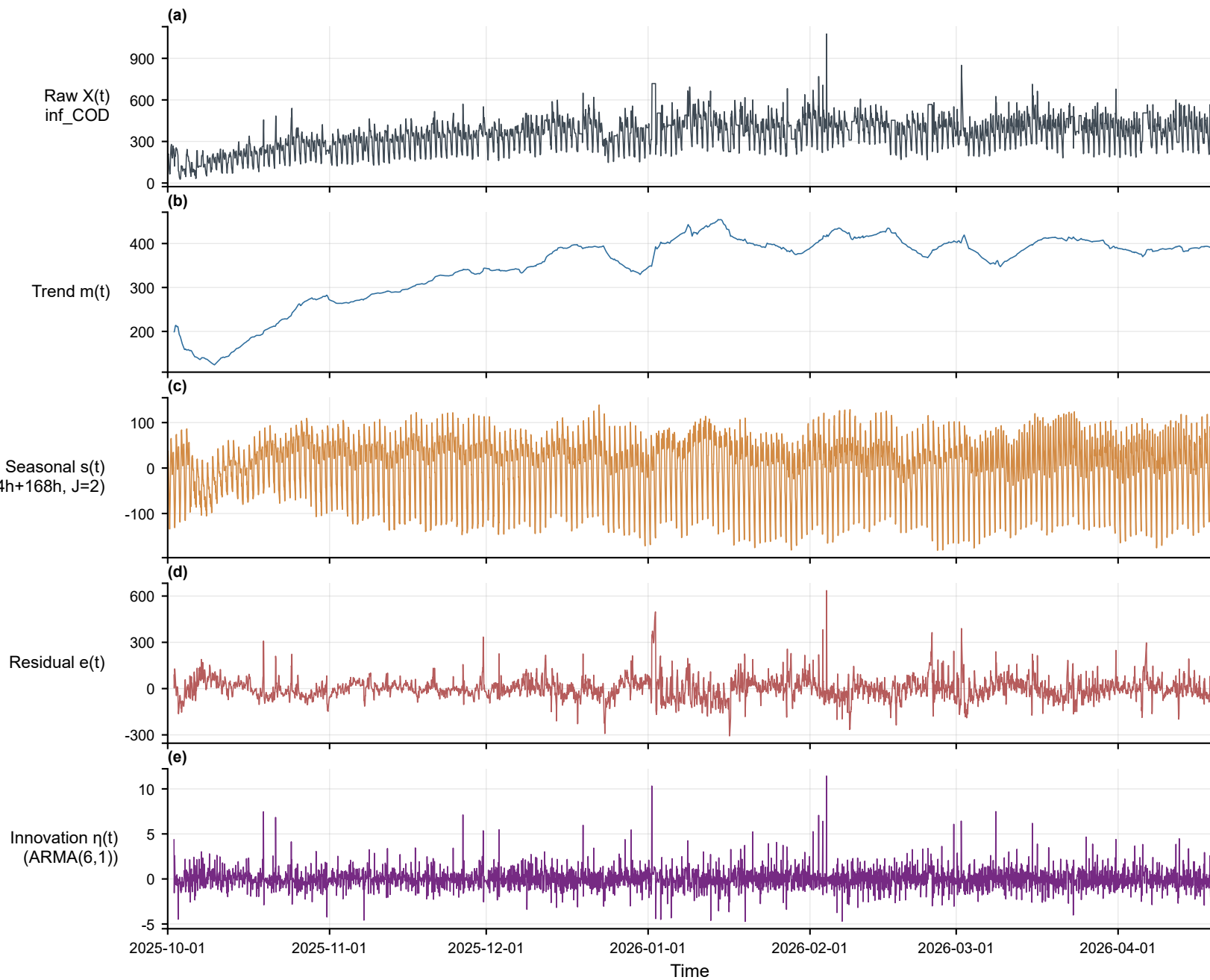
Multi-scale decomposition — inf_COD (influent, hour) [2025-10-01~2026-04-19]
